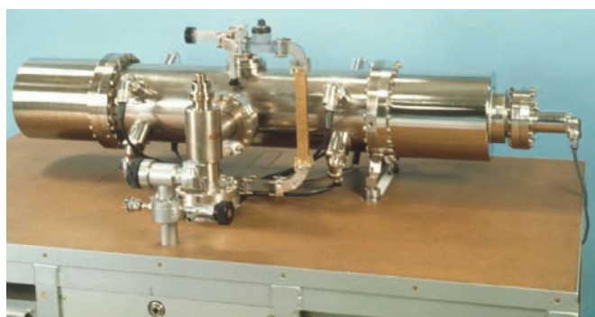
Figure 12. NBS-4.
