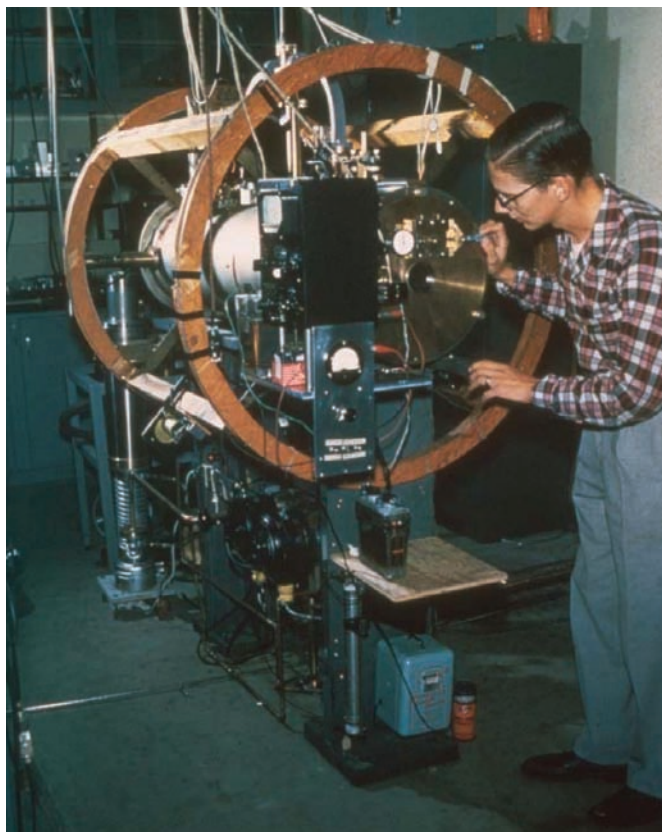
Figure 9. NBS-1.
