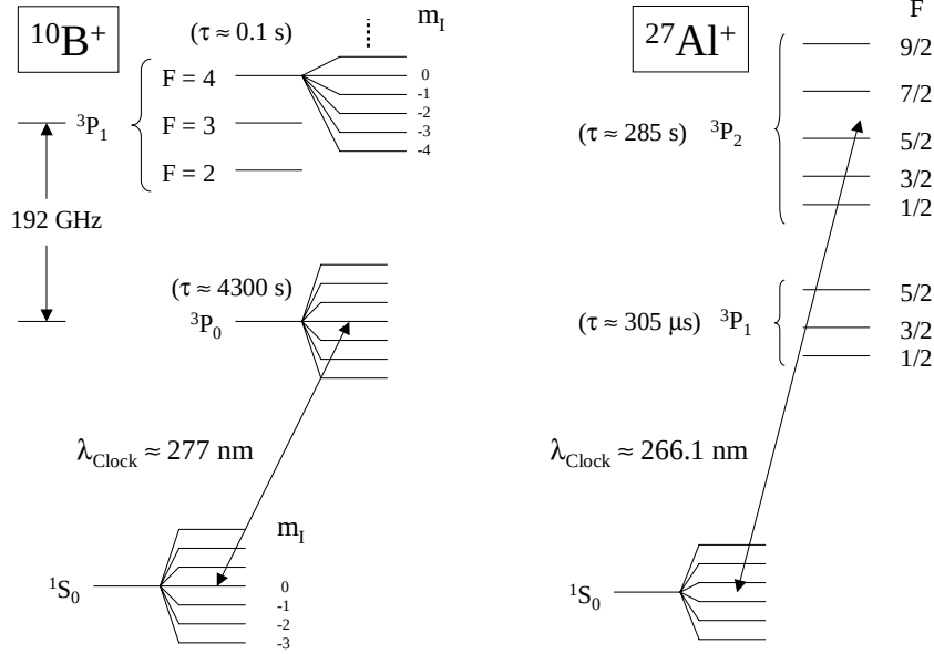
Figure 1. Partial energy-level diagrams for ^{10}\text{B}^+ and ^{27}\text{Al}^+ relevant for potential ion optical clocks. In ^{10}\text{B}^+ , the ^1\text{S}_0(m_I = 0) \rightarrow ^3\text{P}_0(m_I = 0) transition is field-independent for B \rightarrow 0 and has no static electric quadrupole shift. For the ^1\text{S}_0 \rightarrow ^3\text{P}_2 transitions in ^{27}\text{Al}^+ , several are field-independent for B \simeq 100 G; however, it is necessary to average the clock frequency for three equal-magnitude mutually orthogonal directions of the B-field.
